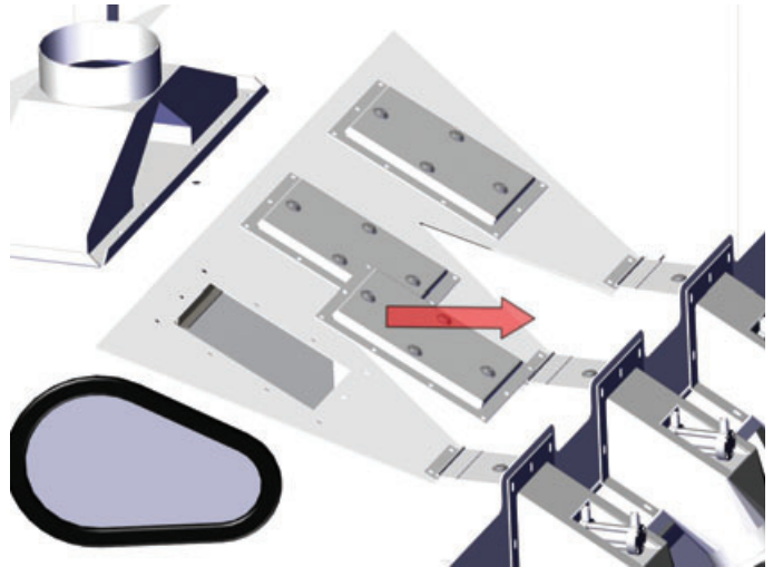
Maintenance access port
