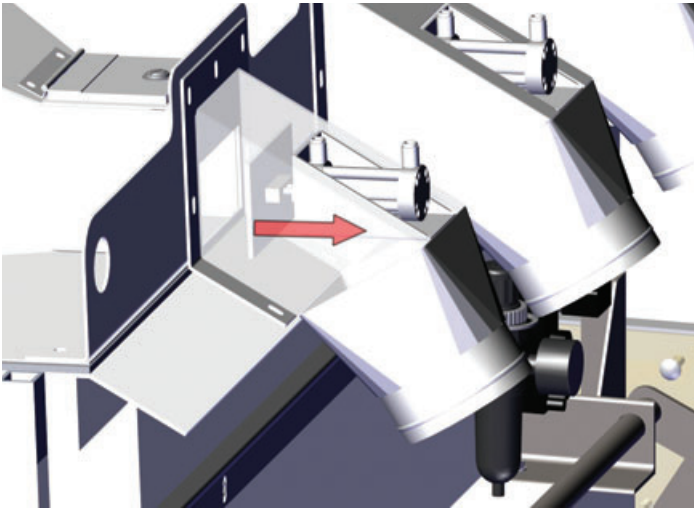
Gate in option position
